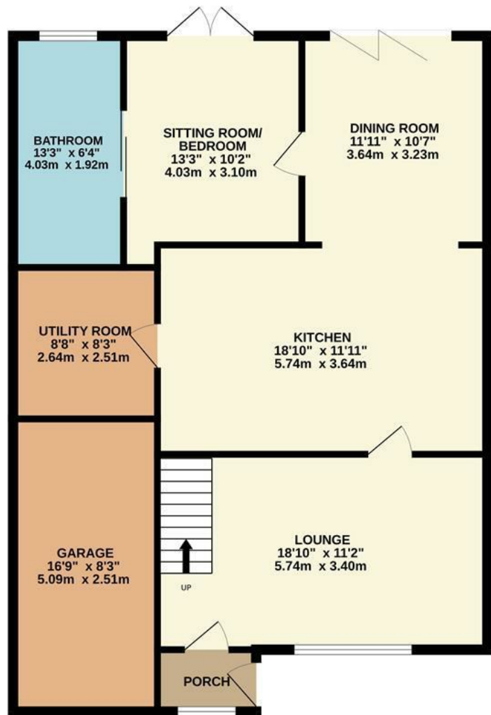
GROUND FLOOR 998 sq.ft. (92.7 sq.m.) approx.
